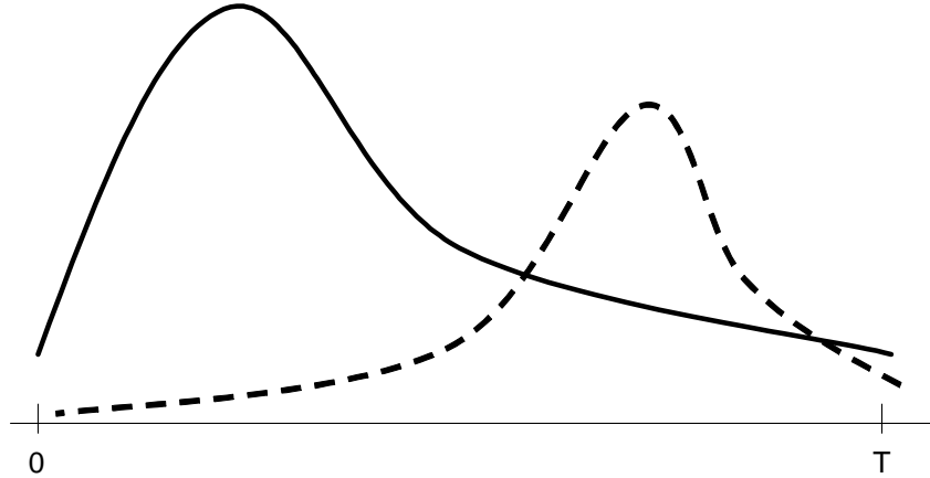
Figure 4. Two utilities whose envelope represents the preference of an agent.
